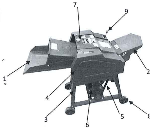
Fig.1. GAJA HITECH AGRO, GJ-C3000, CHAFF CUTTER
